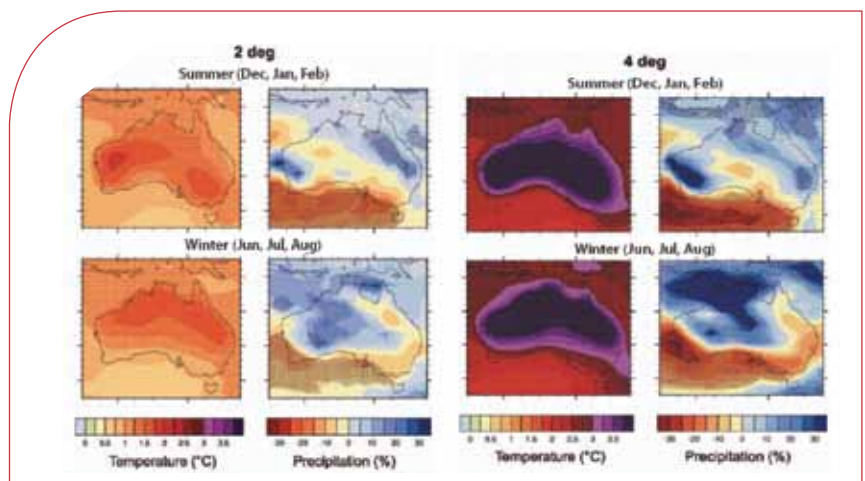
Figure 4. Variability in Temperature and Impacts for Precipitation and Temperature. (PMSEIC 2010)
